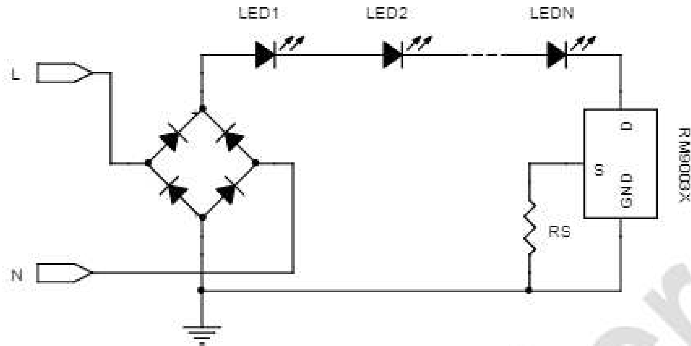
Figure1:single drive
