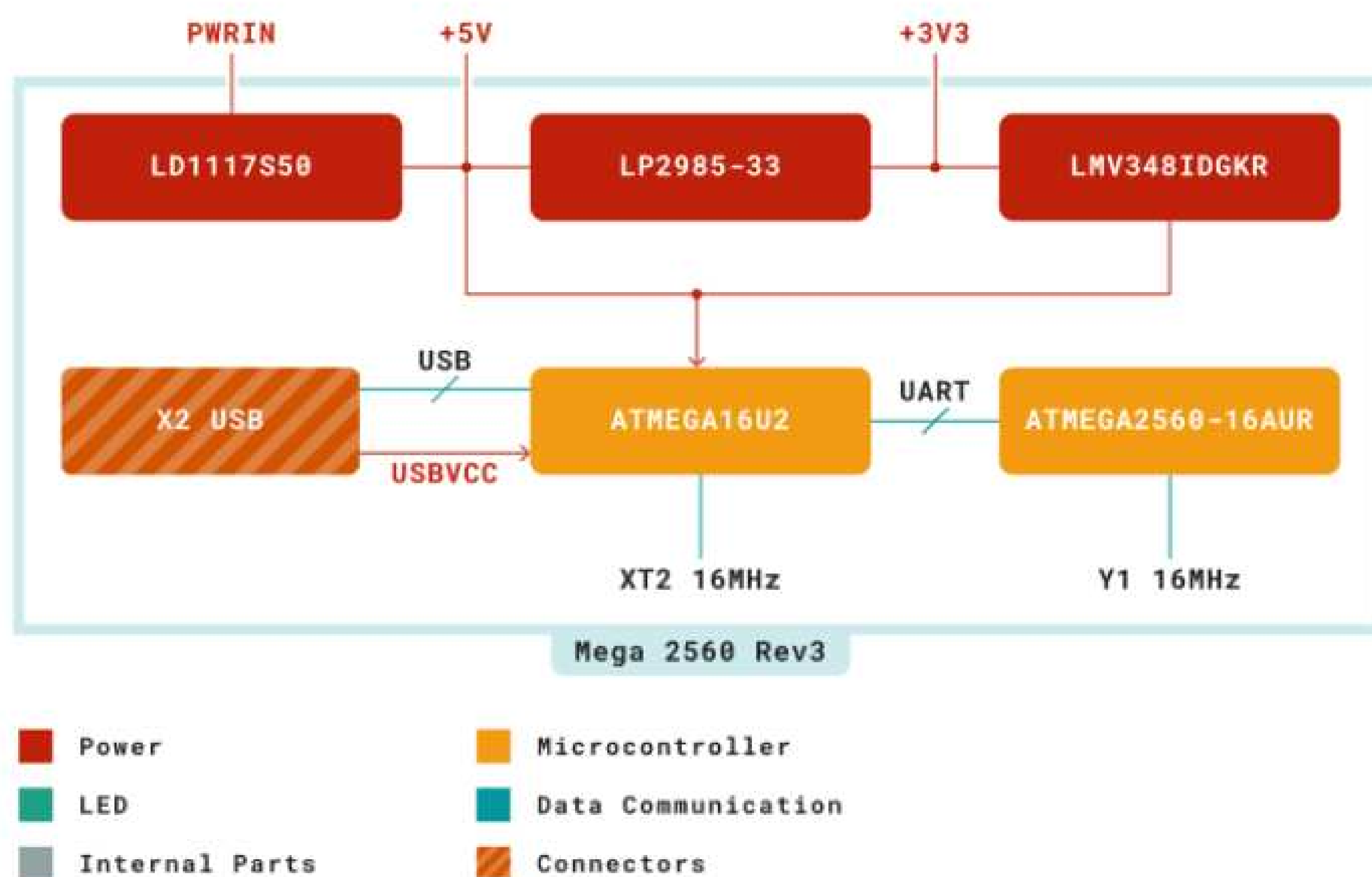
Arduino Mega 2560 Rev3 Block Diagram
