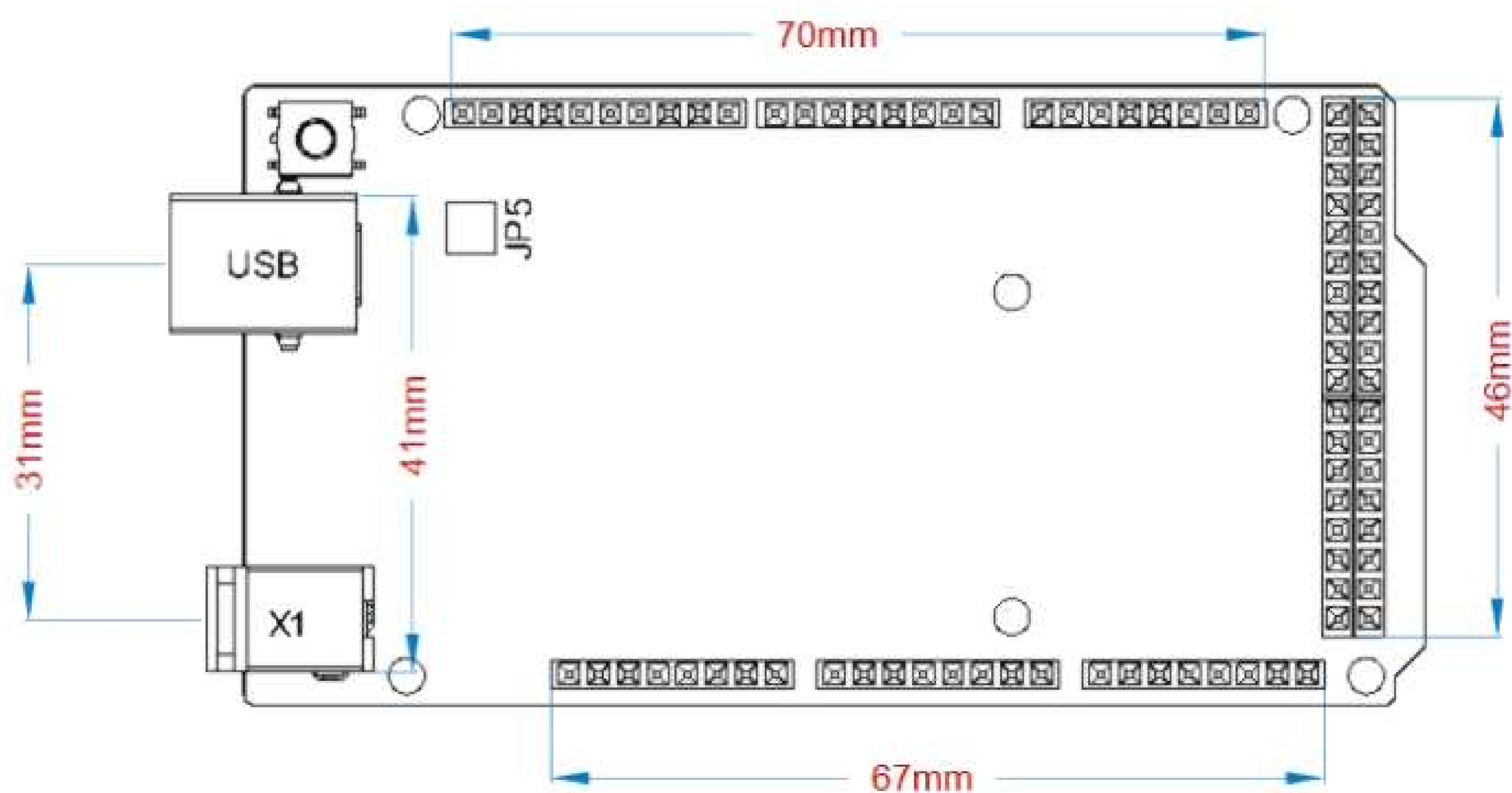
Arduino Mega 2560 Rev3 Mount Holes
